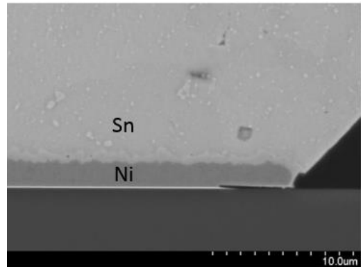
Figure 4: Cross section of the IMC
