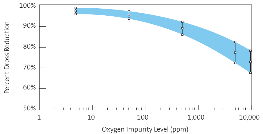
Figure 2: Dross reduction is one of the most important advantages of inert atmosphere wave soldering
